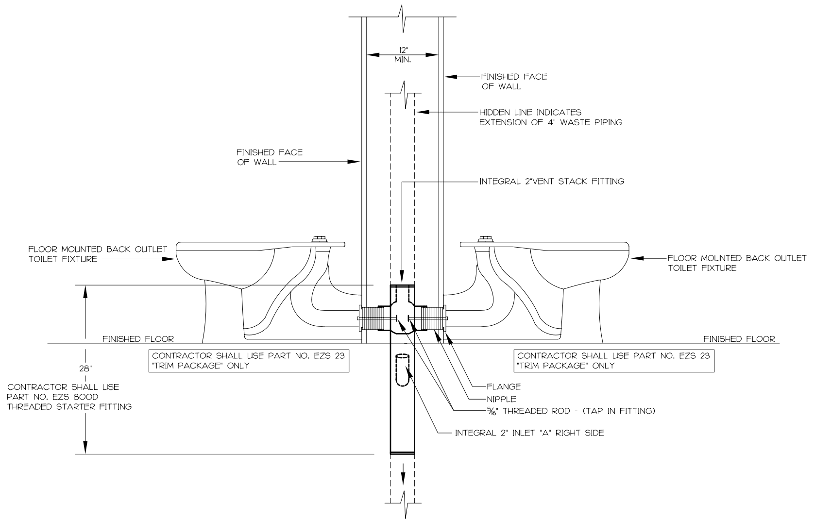
DOUBLE FITTING - LEFT SIDE ELEVATION
