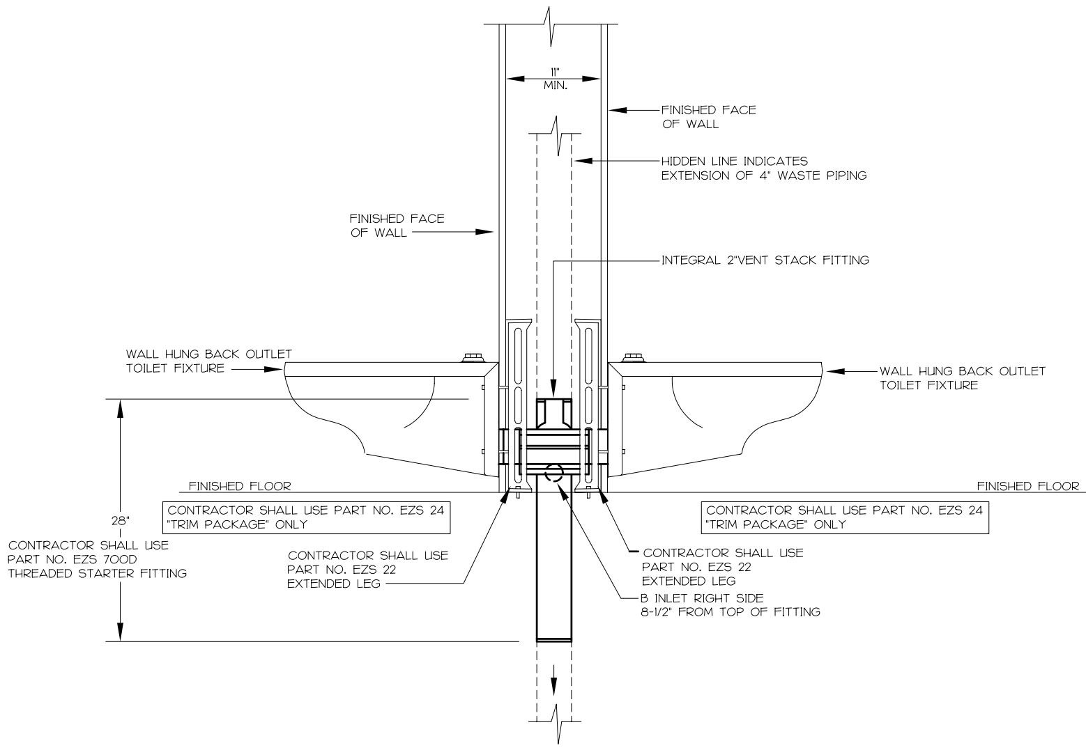
DOUBLE FITTING - LEFT SIDE ELEVATION
