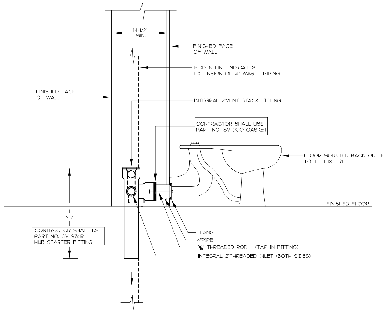
RIGHT HAND FITTING - LEFT SIDE ELEVATION
