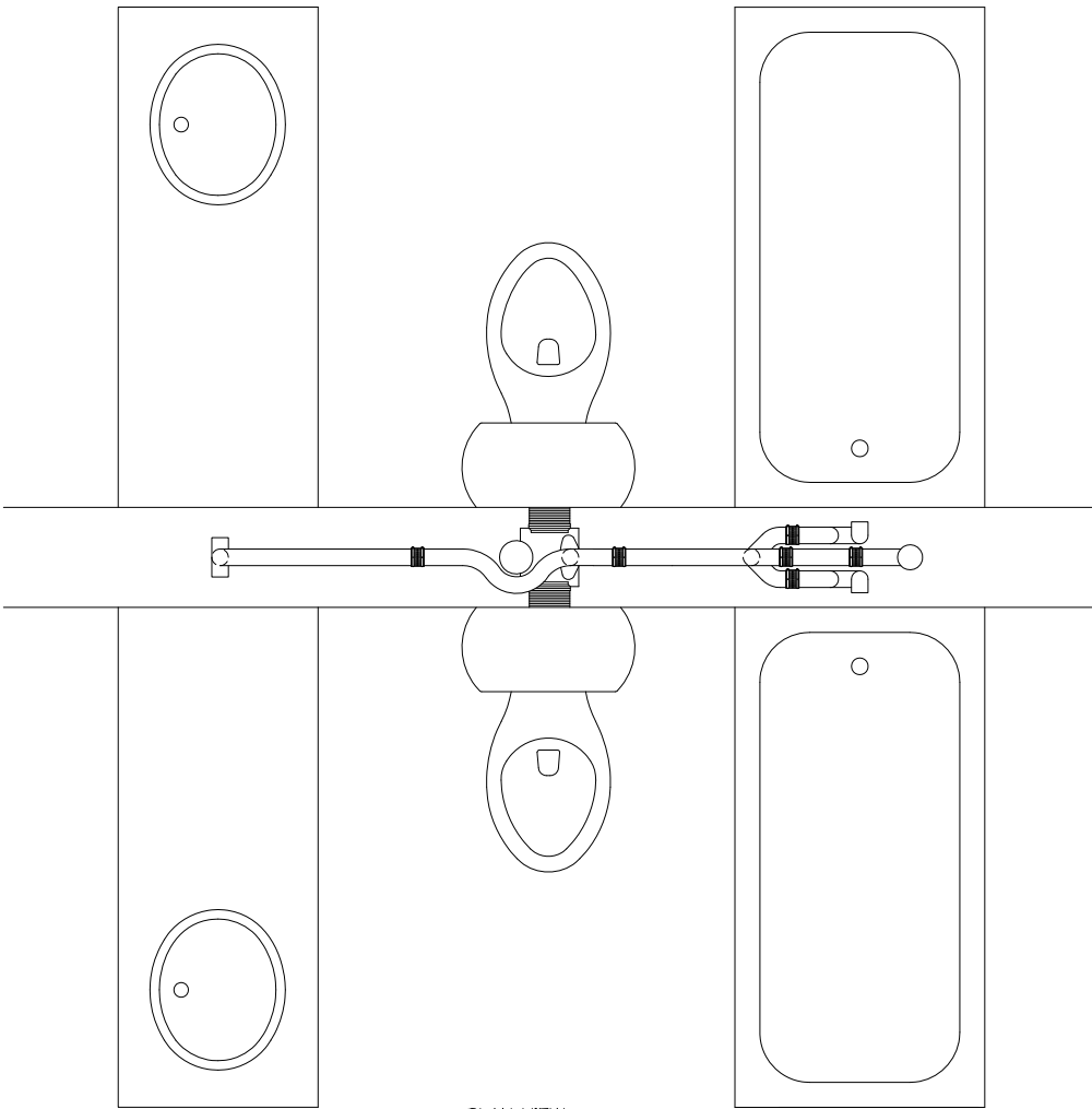
PLAN VIEW
